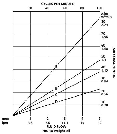
President 10:1 Air Consumption
