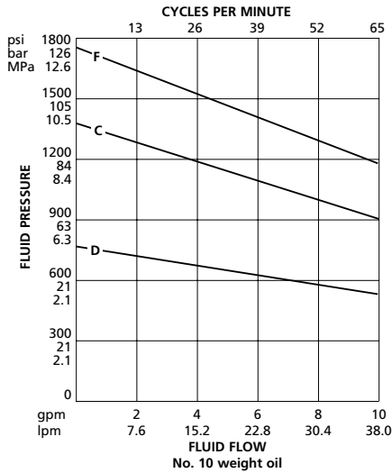
King 20:1 Fluid Flow
