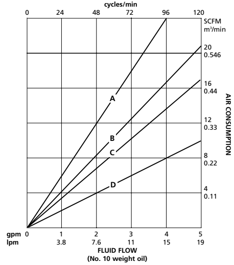
Monark 5:1 Air Consumption
