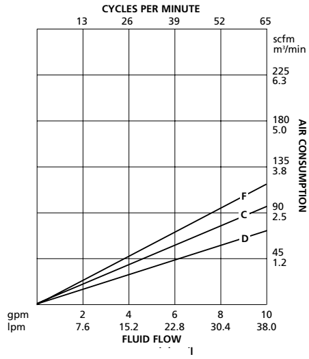
King 20:1 Air Consumption
