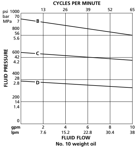
Bulldog 10:1 Fluid Flow
