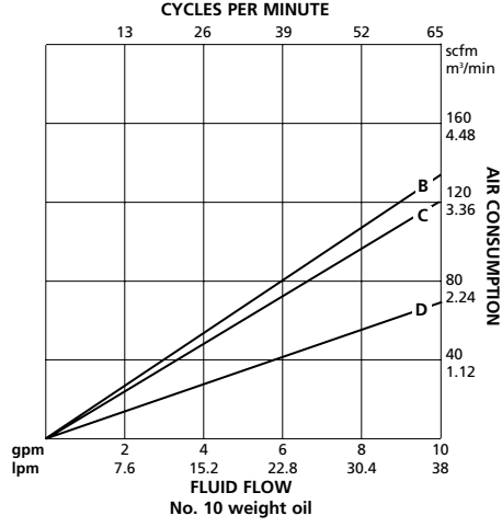
Bulldog 10:1 Air Consumption
