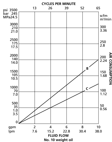
Premier 34:1 Air Consumption
